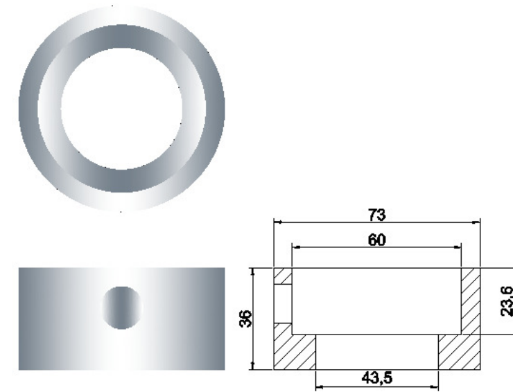
GKMIS_7/1508 8 - 10 DIE HOLDER / SLEEVE
